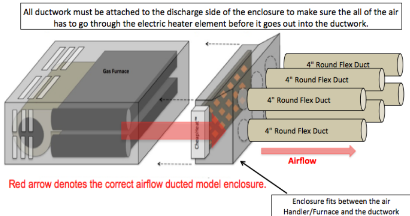
(SA) Style Ducted Enclosure With Ducting Attached
